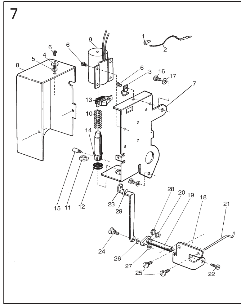
7、WIPER MECHANISM
