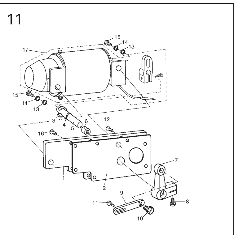
11.AUTOMATIC FOOT LIFTER MECHANISM
