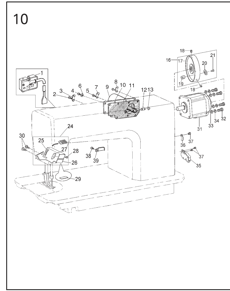
10、REVERSE SEWING AND DETECTOR MECHANISM
